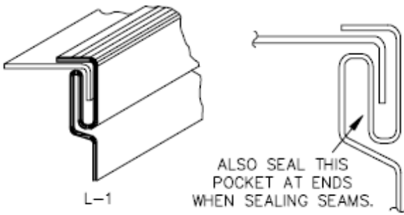
PITTSBURGH LOCK
